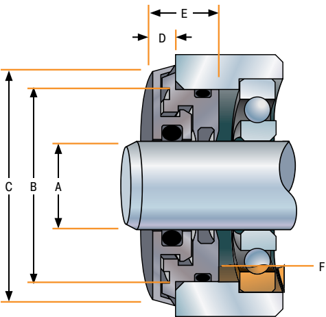
Size Range Table – Standard hardware requirements for shaft, bore and housing.
