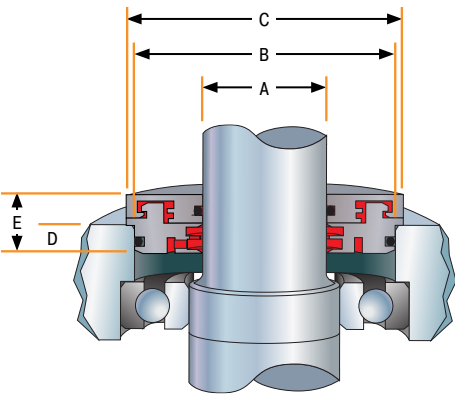
Size Range Table – Standard hardware requirements for shaft, bore and housing.
