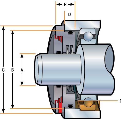
Standard Dimensions
