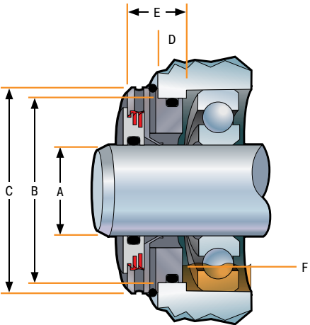
Standard Dimensions
