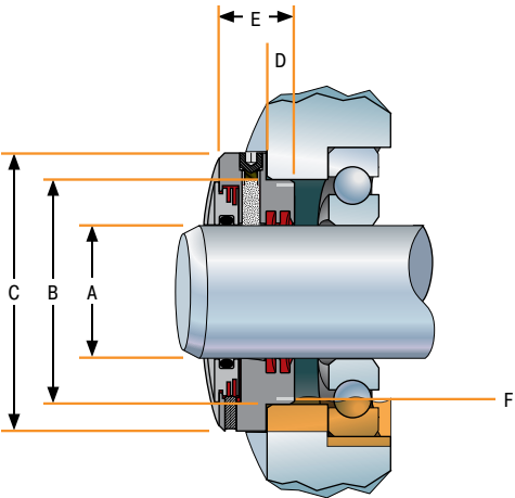
Standard Dimensions
